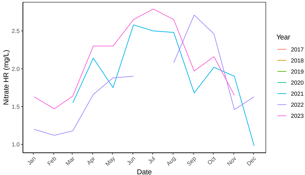
B2 Raceway 2 Nitrate HR (mg/L) Monthly Statistics
